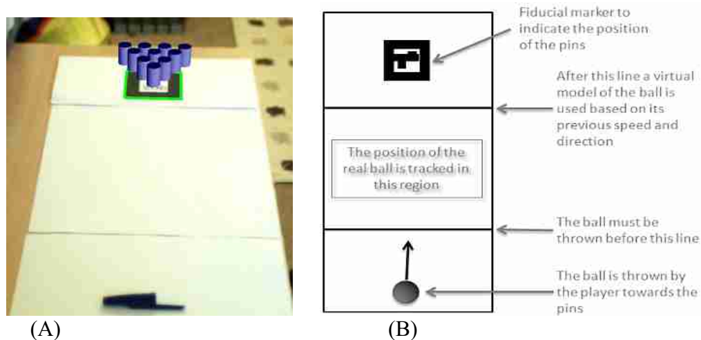
Figure 6: (A) A screenshot of Table-Top MR Bowling and (B) a description of how interaction between the real ball and virtual pins is achieved
